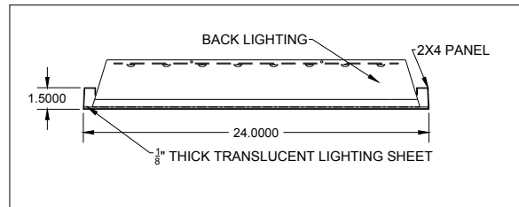
5 PANEL, BACK LIGHT & LIGHTING SHEET CUT SECTION N.T.S.
