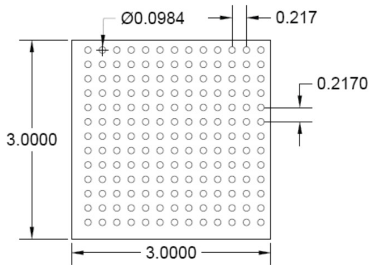
PATTERN M 0.098" DIA Holes x 0.217" Spacing Straight Centers
