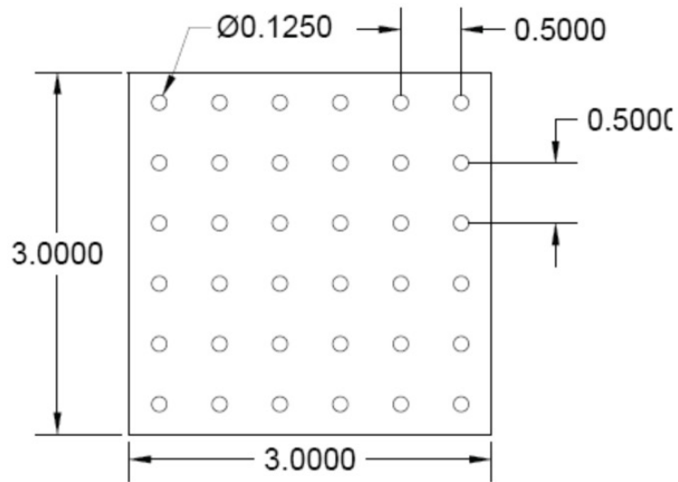
PATTERN V 0.125" DIA Holes x 0.50" Spacing Straight Centers
