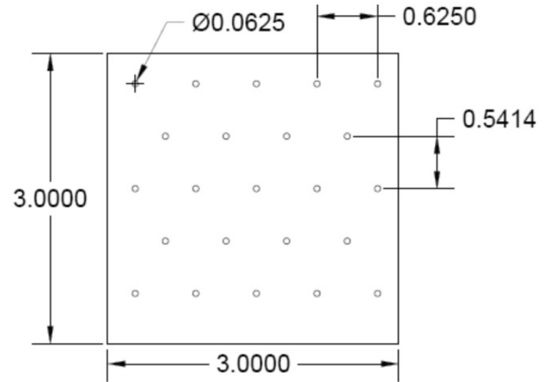
PATTERN K 0.063" DIA Holes x 0.625" Spacing Staggered Centers
