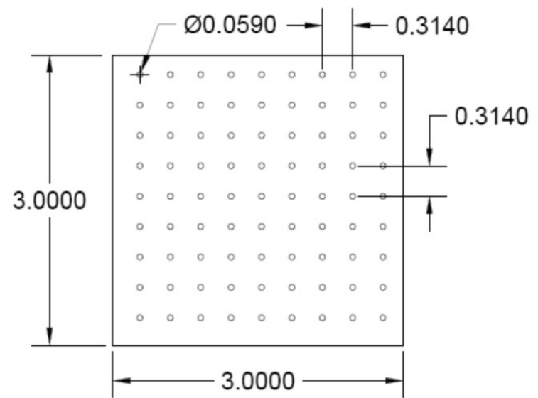
PATTERN D 0.059" DIA Holes x 0.314" (8mm) Spacing Straight Centers
