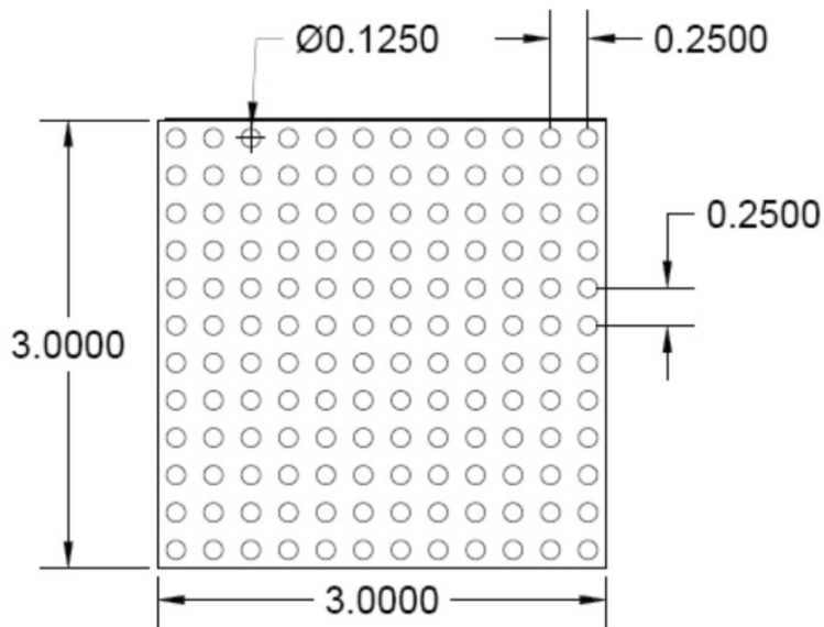
PATTERN R 0.125" DIA Holes x 0.25" Spacing Straight Centers
