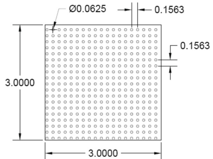
PATTERN H 0.063" DIA Holes x 0.1563" Spacing Straight Centers
