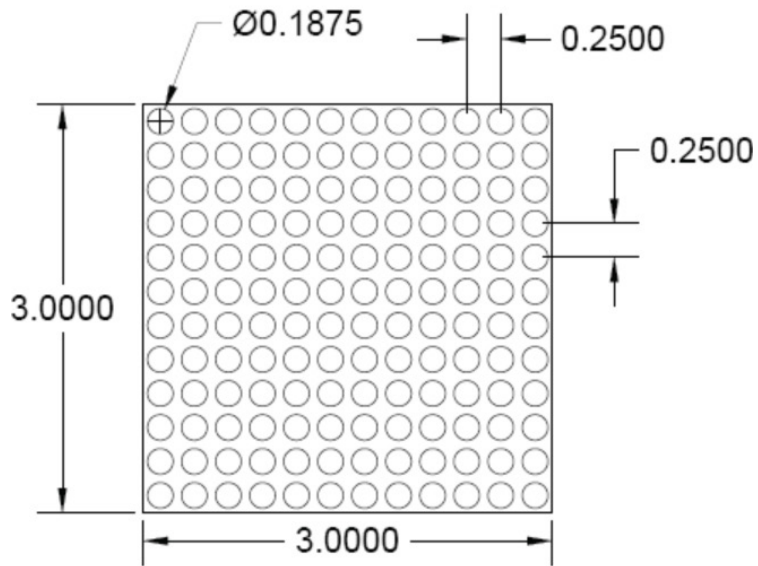
PATTERN Z 0.1875" DIA Holes x 0.25" Spacing Straight Centers
