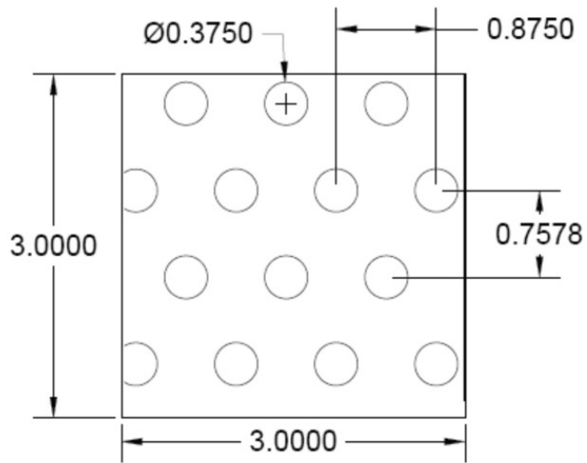
PATTERN HH 0.375" DIA Holes x 0.875" Spacing Straight Centers
