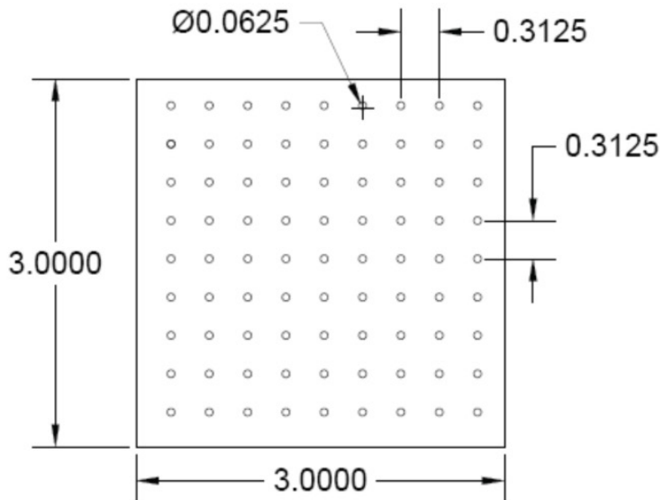
PATTERN J 0.063" DIA Holes x 0.3125" Spacing Straight Centers
