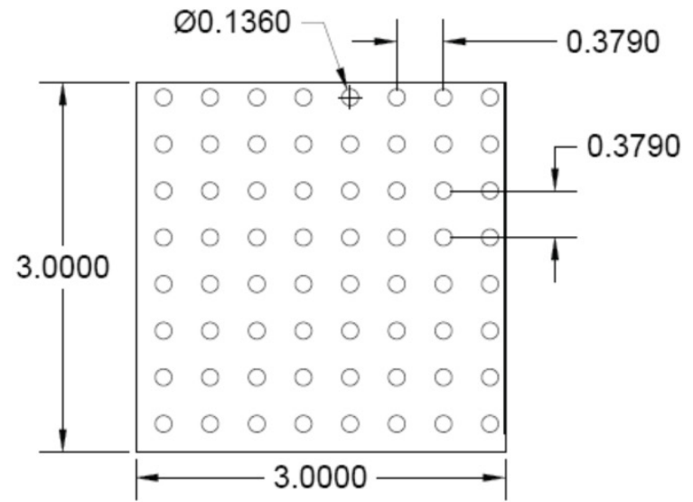
PATTERN W 0.136" DIA Holes x 0.379" Spacing Straight Centers
