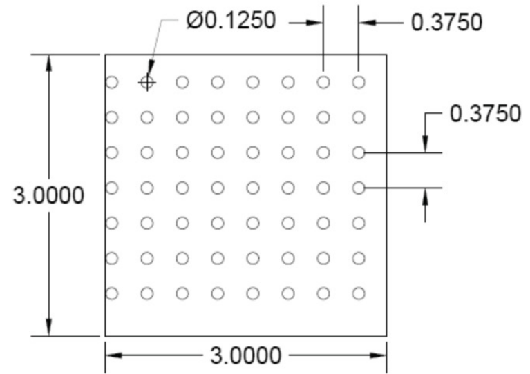
PATTERN T 0.125" DIA Holes x 0.375" Spacing Straight Centers
