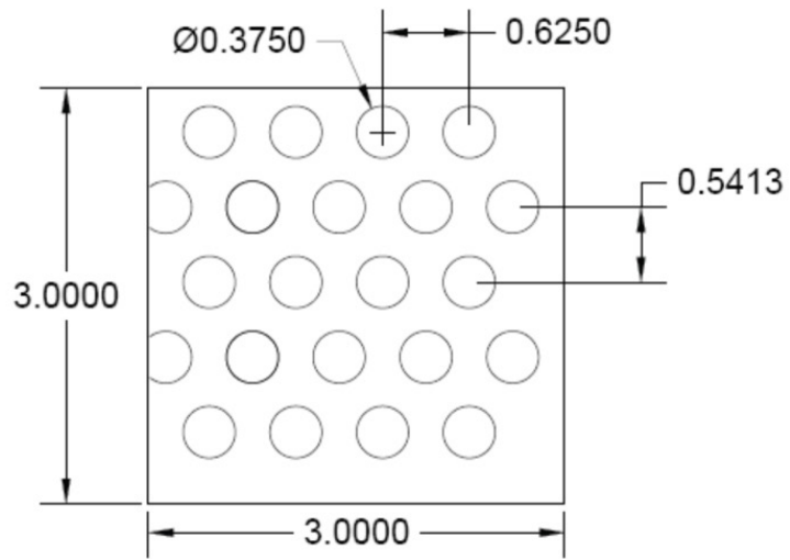
PATTERN GG 0.375" DIA Holes x 0.625" Spacing 60 Degree Staggered Centers
