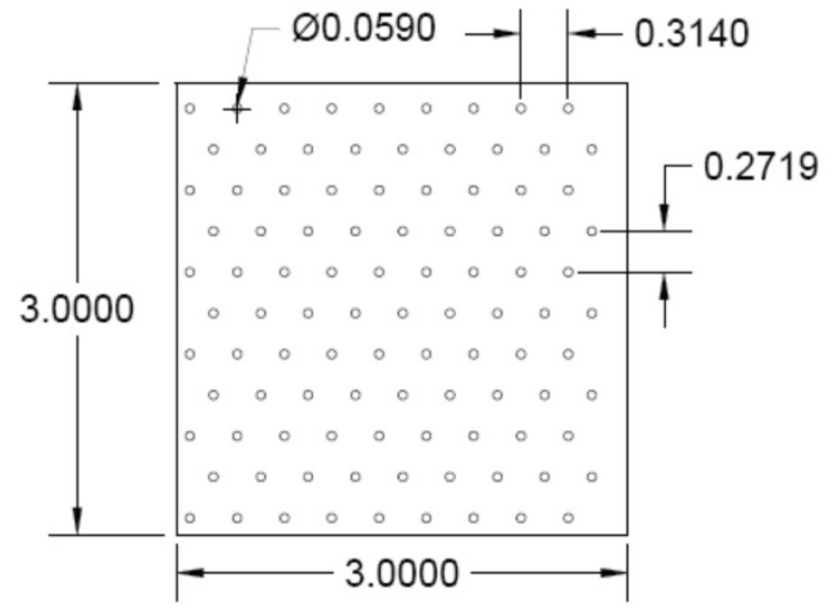
PATTERN C 0.059" DIA Holes x 0.314" (8mm) Spacing 60 Degree Staggered Centers
