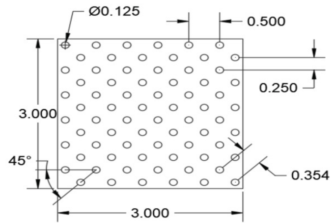
PATTERN S 0.125" DIA Holes x 0.500" Spacing 45 Degree Staggered Centers
