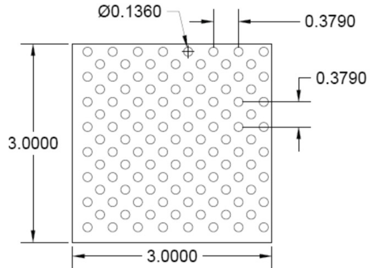
PATTERN X 0.136" DIA Holes x 0.379" Spacing Staggered Centers
