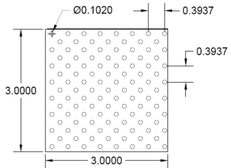
PATTERN P 0.102" DIA Holes x 0.3937" Spacing Staggered Centers
