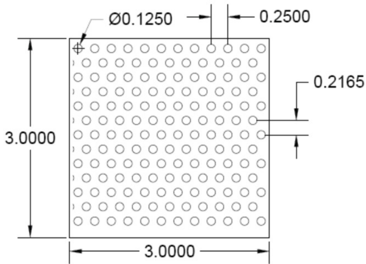
PATTERN Q 0.125" DIA Holes x 0.25" Spacing 60 Degree Staggered Centers
