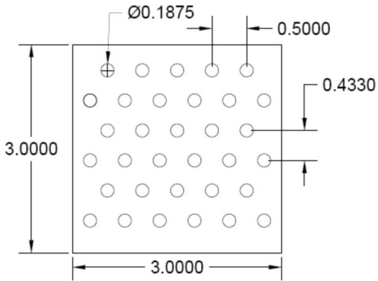
PATTERN CC 0.1875" DIA Holes x 0.50" Spacing 60 Degree Staggered Centers
