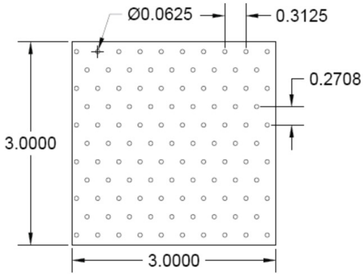
PATTERN I 0.063" DIA Holes x 0.3125" Spacing 60 Degree Staggered Centers
