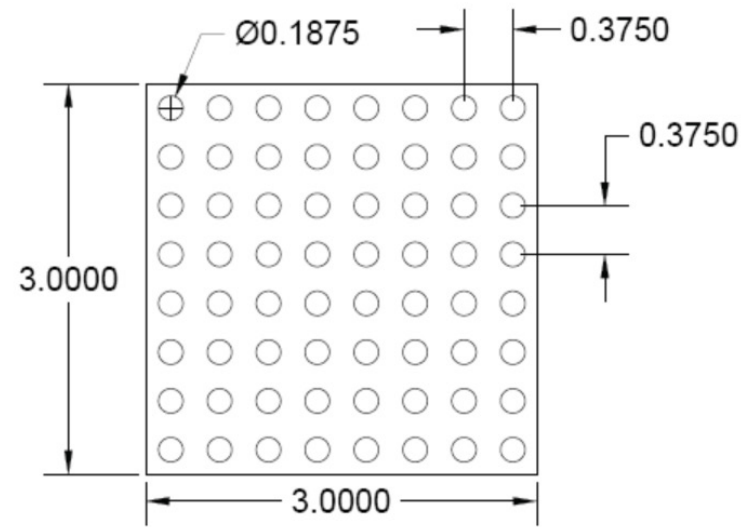
PATTERN AA 0.1875" DIA Holes x 0.375" Spacing Straight Centers
