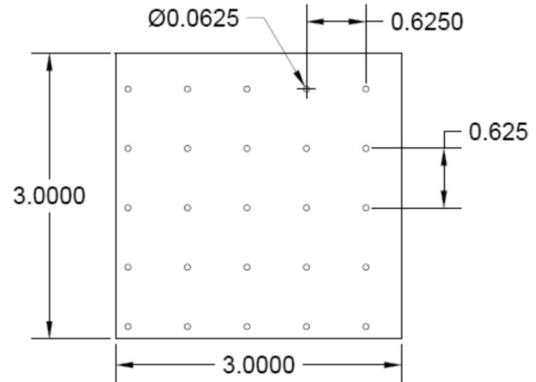
PATTERN L 0.063" DIA Holes x 0.625" Spacing Straight Centers
