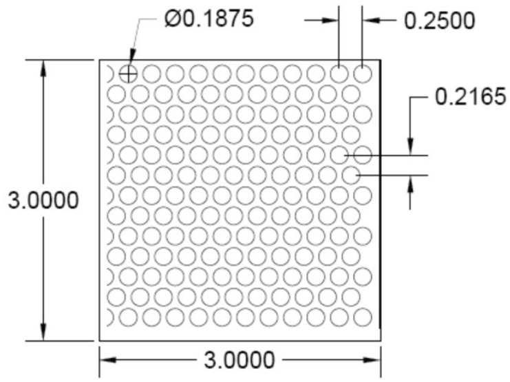
PATTERN Y 0.1875" DIA Holes x 0.25" Spacing 60 Degree Staggered Centers
