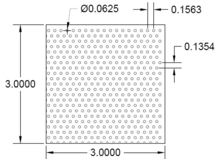
PATTERN G 0.063" DIA Holes x 0.1563" Spacing 60 Degree Staggered Centers
