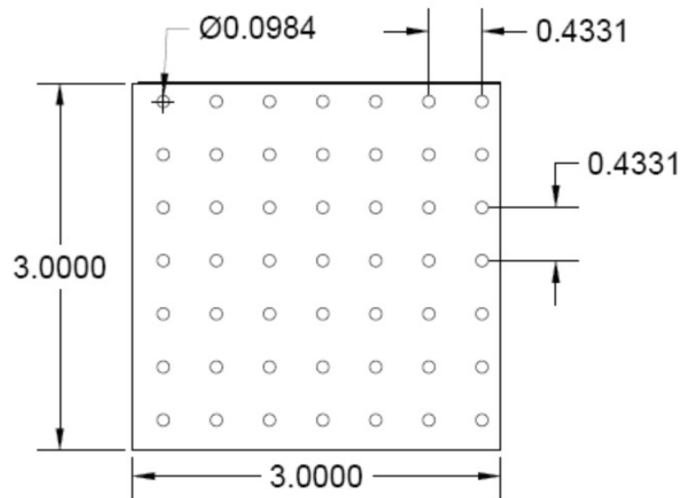
PATTERN N 0.098" DIA Holes x 0.4331" Spacing Straight Centers
