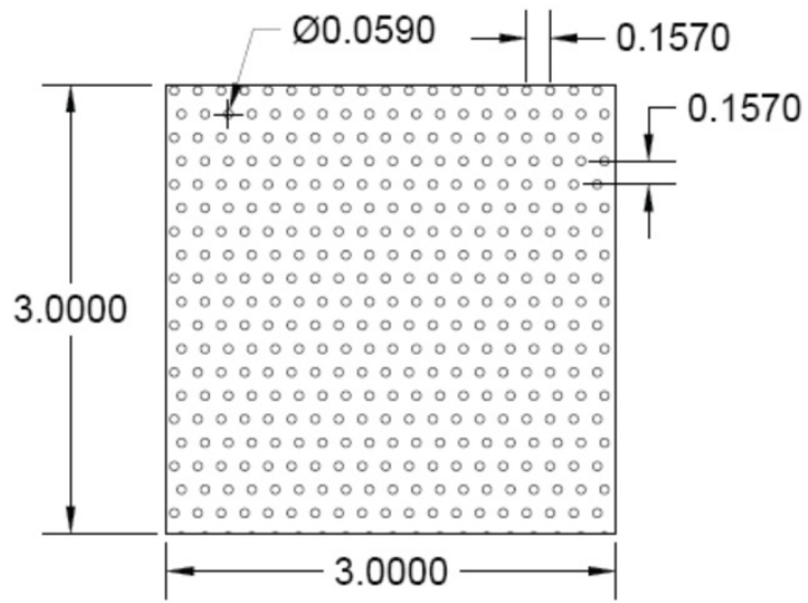
PATTERN A 0.059" DIA Holes x 0.157" (4mm) Spacing 60 Degree Staggered Centers
