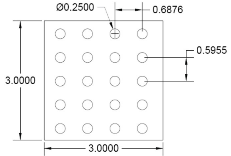
PATTERN EE 0.25" DIA Holes x 0.596" Spacing Straight Centers
