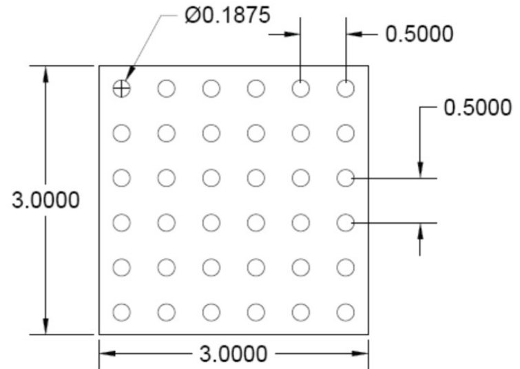
PATTERN BB 0.1875" DIA Holes x 0.50" Spacing Straight Centers
