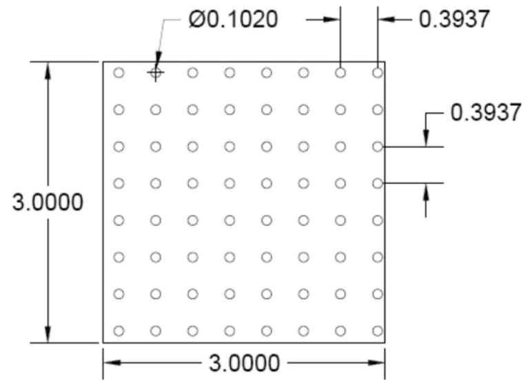
PATTERN O 0.102" DIA Holes x 0.3937" Spacing Straight Centers
