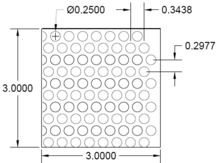
PATTERN DD 0.25" DIA Holes x 0.348" Spacing 60 Degree Staggered Centers
