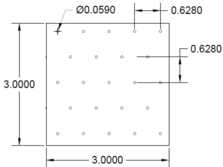
PATTERN F 0.059" DIA Holes x 0.628" Spacing Staggered Centers
