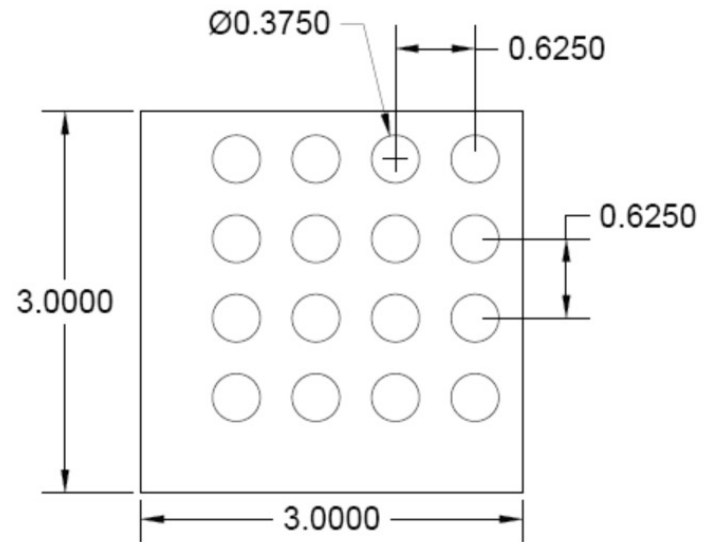
PATTERN FF 0.375" DIA Holes x 0.625" Spacing Straight Centers
