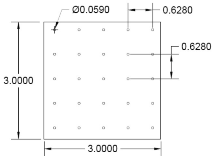
PATTERN E 0.059" DIA Holes x 0.628" Spacing Straight Centers
