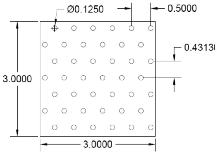
PATTERN U 0.125" DIA Holes x 0.50" Spacing 60 Degree Staggered Centers
