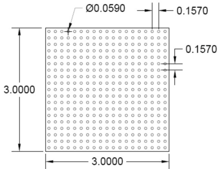
PATTERN B 0.059" DIA Holes x 0.157" (4mm) Spacing Straight Centers
